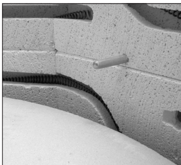
Keep ware and shelves at least 1" away from the thermocouple.
