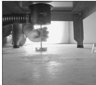
Installing the Orton Master Vent. The fan and fan housing are separate from the air intake cup shown above.
