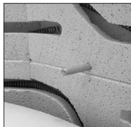
Keep shelves and ware at least 1" away from the thermocouple or Kiln Sitter tube.
