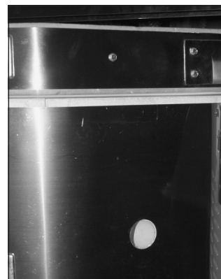
The light around the edge of the lid and inside the peephole changes color as the kiln gets hotter. You can learn to estimate temperature by the color of that light.
