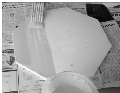
Applying kiln wash with a haik brush.
