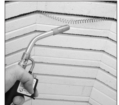
Using a propane torch with push button igniter to heat a bulging element.
